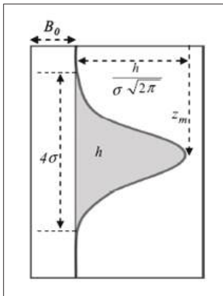
Figure 3. Shifted Gaussian distribution showing four parameters ( B_0 , h , \sigma and z_m ), used to describe Chl-a vertical profiles (Siswanto et al. 2005).
